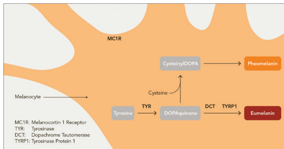
Figure 1: Melanin synthesis
